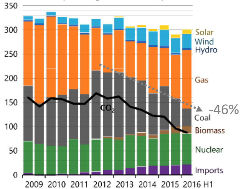
Demand (TWh/yr) + CO 2 emissions (MT/yr)
